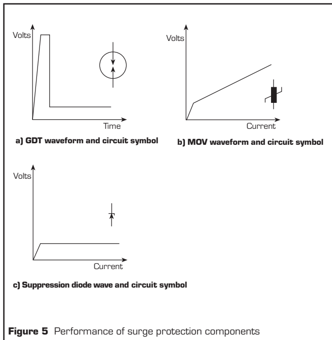
Figure 5 Performance of surge protection components
