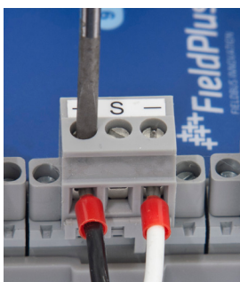
Figure 5.1: Screw Terminal
