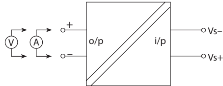
Figure 8.2: Loop powered DO test circuit
