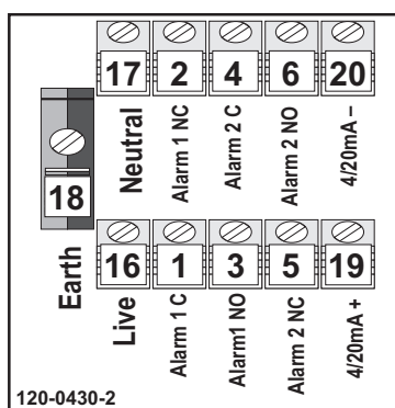
Figure 8- K1550FX terminals
