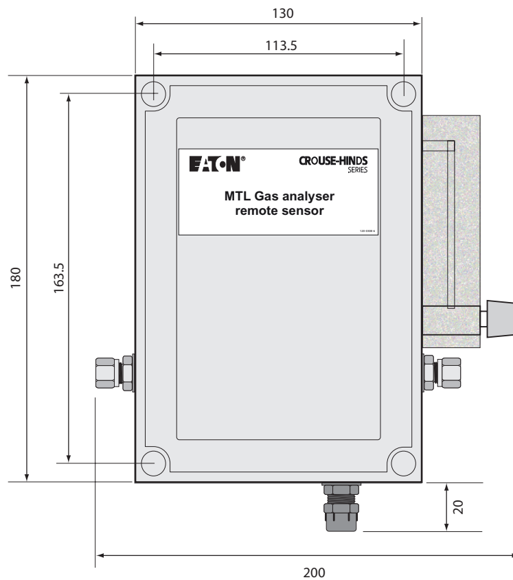
Figure 3a- Enclosure- nylon piping version
