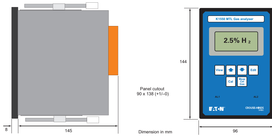
Figure 1- General layout
