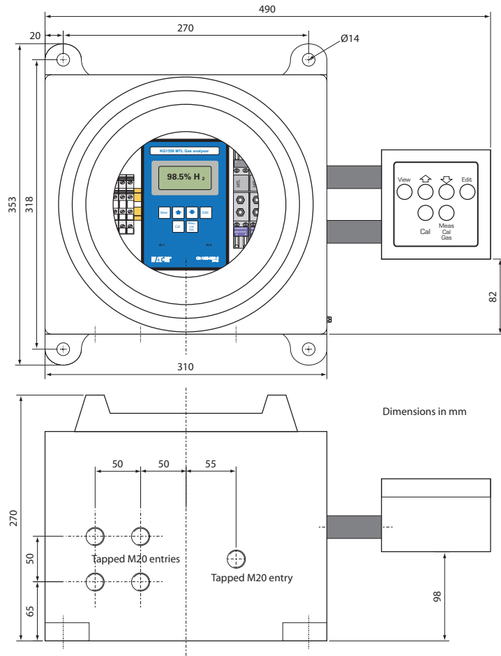
Figure 2- K1550 in Ex d enclosure
