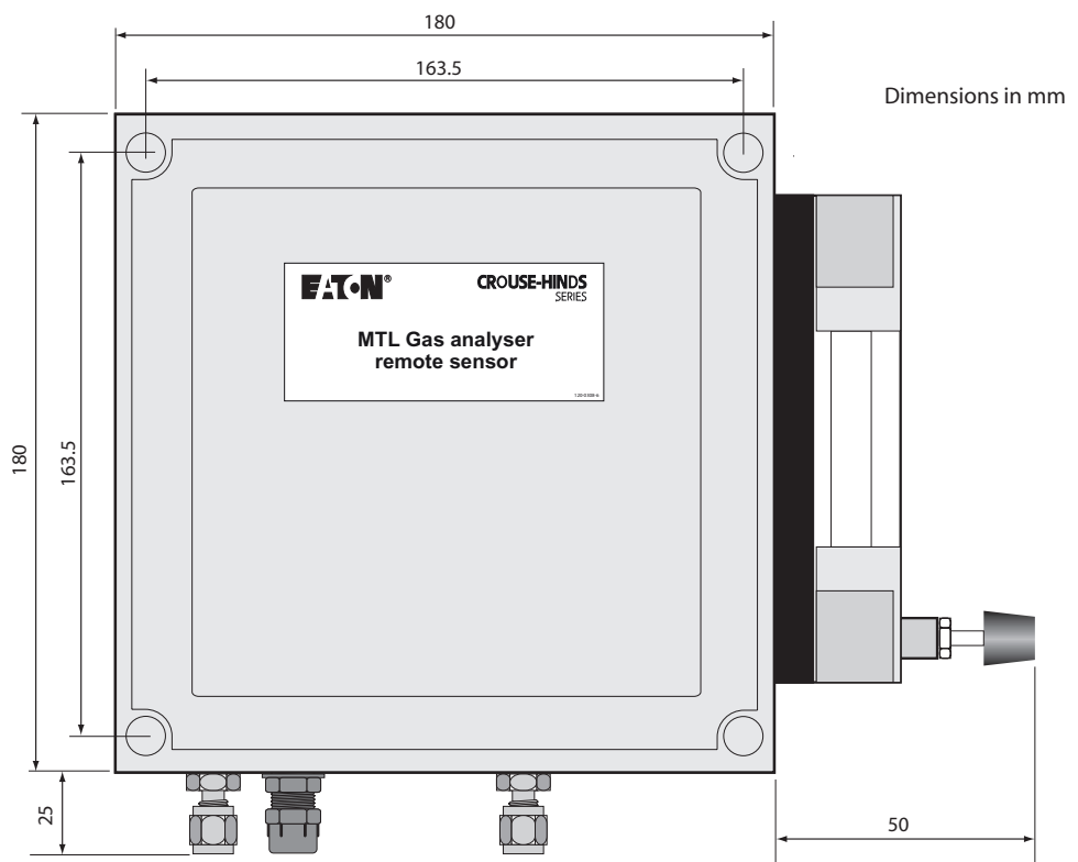
Figure 3b- Enclosure- stainless steel piping version
