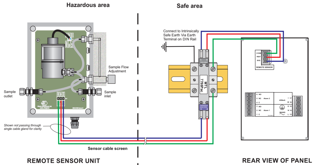
Figure 5- Connections when sensor is in a hazardous area
