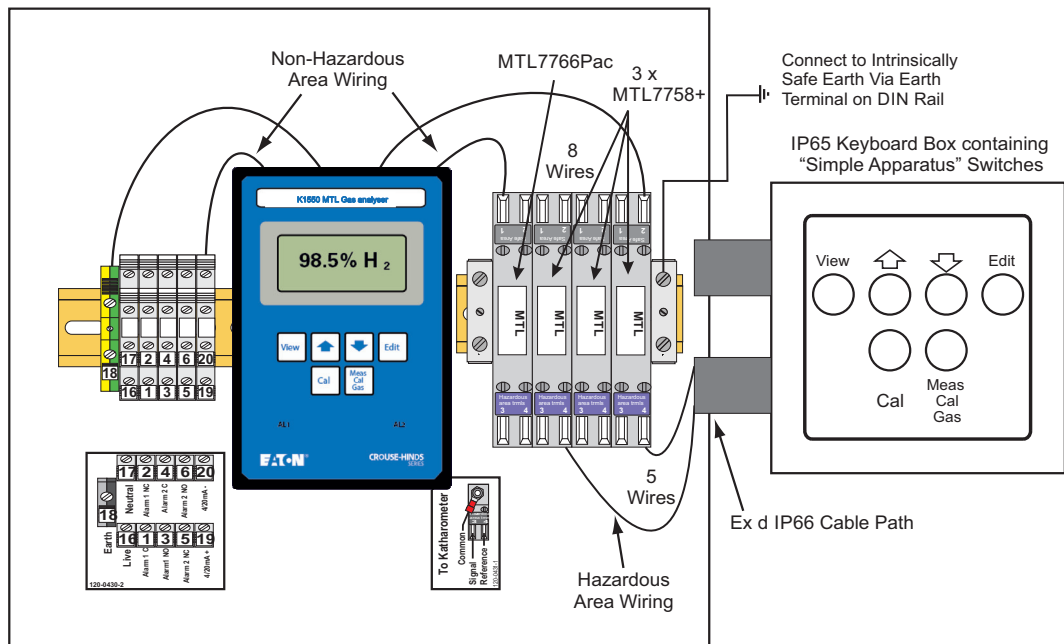
Figure 6 - Internal wiring for K1550FX model mounted in a hazardous area
