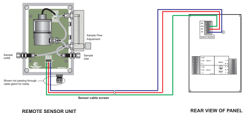
Figure 4- Connections for installation in non-hazardous area
