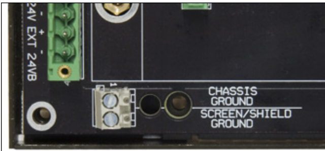
Figure 5.9 - Ground terminals
