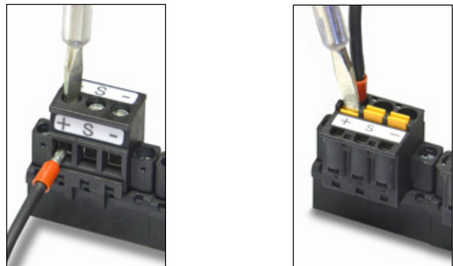
Figure 5.8 - Screw terminal and spring-clamp connectors
