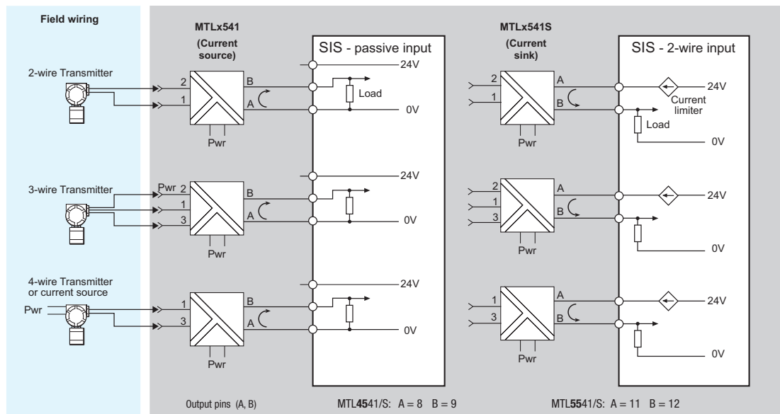
Figure 1.1 – Analogue Input Connections
