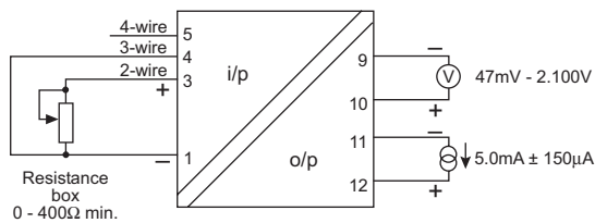
Figure 8.10: AI test circuit #5 "Resistance input"
