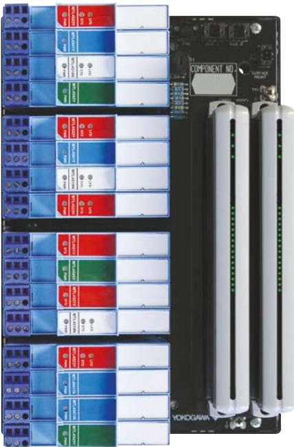
Left wiring model
