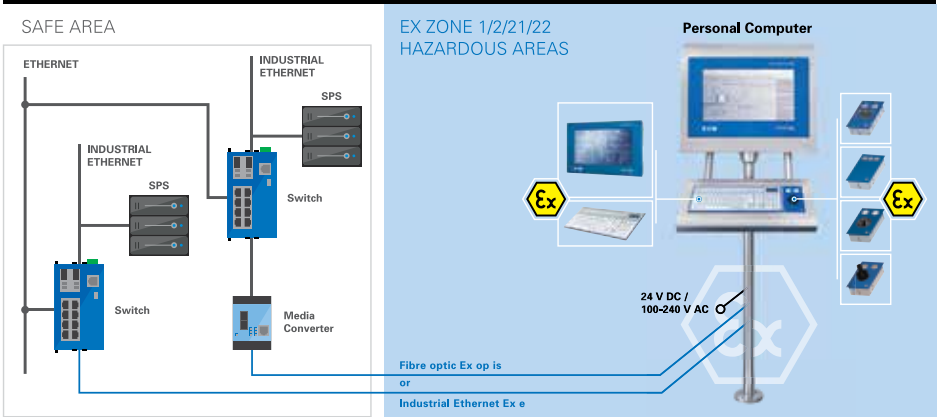
MTL GECMA PC operating principle
