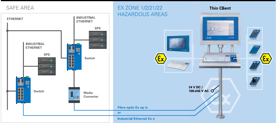
MTL GECMA TC operating principle
