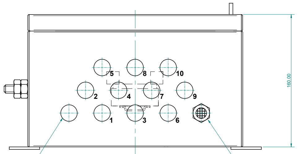
VIEW SHOWING POSITION OF CABLE GLAND AND BREATHER. GLAND NOT SHOWN FOR CLARITY
