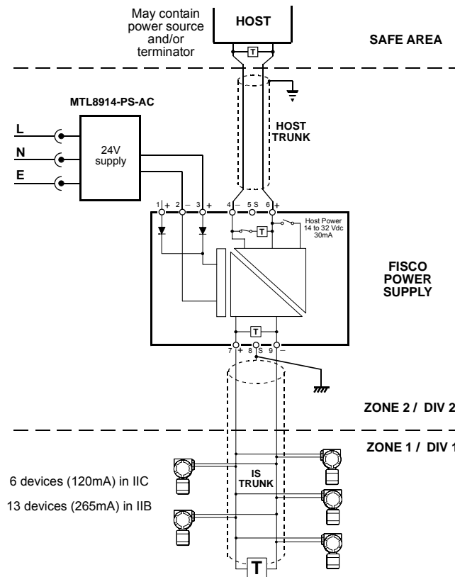
Figure 25 - Fieldbus power supply installed in Zone 2 or Division 2
