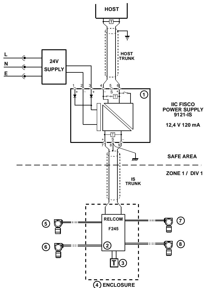
Figure 27 - Typical installation
