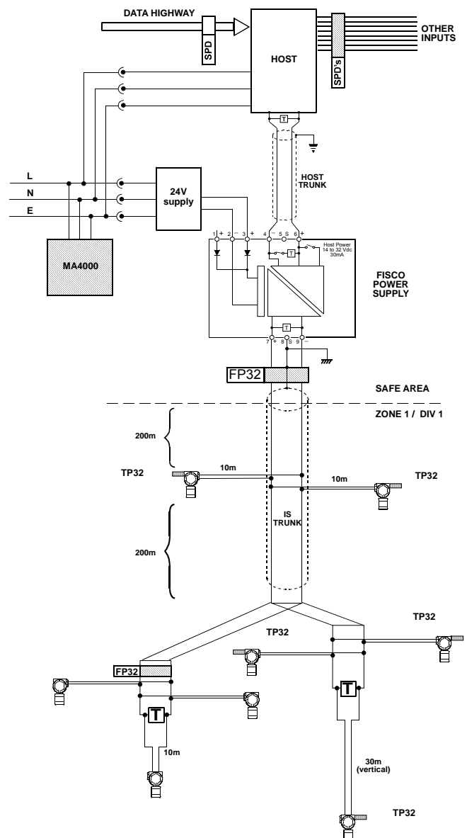
Figure 24 - Adequately protected Fieldbus system
