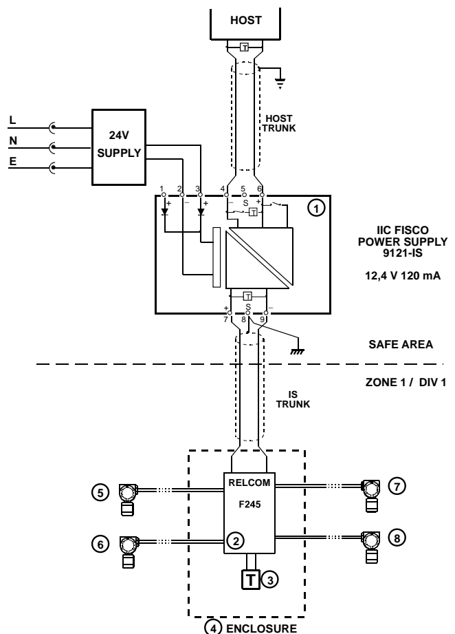
Figure 27 - Typical installation
