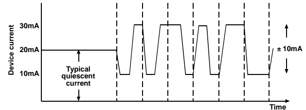
Figure 5 - Idealised current waveform of field device
